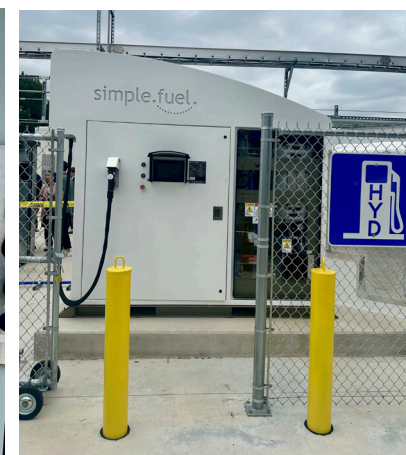
Operational fuel station at J.J. Pickle Research Campus, the University of Texas in Austin.
